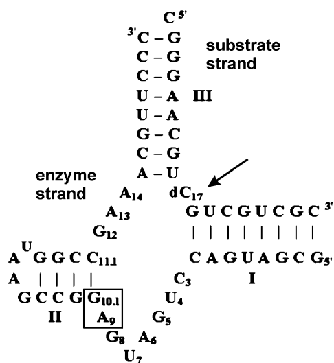
Figure 1. Secondary structure of the hammerhead ribozyme used in our studies. The cleavage site is indicated by the arrow. The position of the Mn^{II} binding site as found in the crystal structure [10c] is marked by the box.
