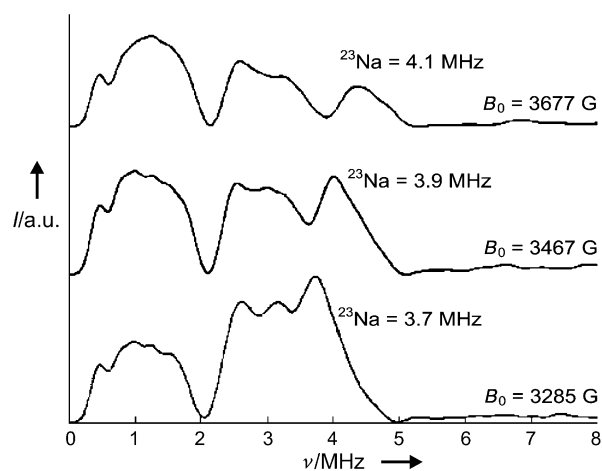
Figure 5. Fourier-transformed two-pulse ESEEM spectra at different field positions (given in the figure) of a sample with 0.2 mM ribozyme, 0.2 mM Mn II , and 1 M NaCl in phosphate buffer. The other experimental parameters were: T = 4 \text{ K} , pulse lengths for both pulses were 12 ns, the attenuation was set to 5 dB by use of a 1 kW TWT, \tau_{\text{start}} was 104 ns, the increments of \tau were 8 ns, the shot repetition time was 10 ms, and 100 scans were accumulated. I, amplitude of the power Fourier transformation in arbitrary units (a.u.); \nu , frequency (MHz).
