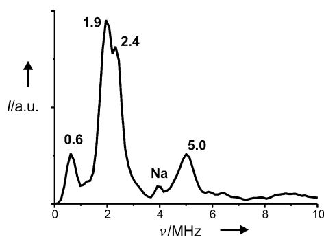
Figure 6. Skyline projection of a 2D three-pulse ESEEM spectrum from a sample with 0.2 mM ribozyme, 0.2 mM Mn II , and 1 M NaCl in phosphate buffer. The other experimental parameters were: T = 4 K, pulse lengths for all three pulses were 12 ns, the attenuation was set to 7 dB by use of a 1 kW TWT, \tau_{\text{start}} was 136 ns, T_{\text{start}} was 16 ns, T and \tau were incremented in 8-ns steps, the dimensions of the array were 64 points by 256 points for T and \tau respectively, B_0 = 3466 G. The shot repetition time was 10 ms, and 100 scans were accumulated. I , amplitude of the power Fourier transformation in arbitrary units (a.u.); \nu , frequency.
