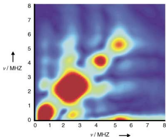
Figure 7. The (+, +) quadrant of the HYSORE spectrum of the Mn II high-affinity binding site in the region of the nitrogen couplings, recorded on a sample with 0.2 mM ribozyme, 0.2 mM Mn II , and 1 M NaCl in phosphate buffer. The other experimental parameters were: T = 4 K, the pulse lengths for the three \pi /two-pulses were 12 ns and for the inversion pulse 24 ns, \tau_{\text{start}} was 204 ns, t_{1,\text{start}} was 16 ns, t_{2,\text{start}} was 28 ns, and t_1 and t_2 were incremented in 8-ns steps, the dimensions of the array were 200 points by 200 points for t_1 and t_2 , respectively, B_0 = 3466 G. The shot repetition time was 8 ms, and 70 scans were accumulated. \nu , frequency in MHz.
